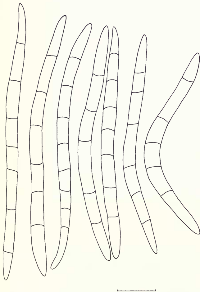
Fig. 48 Ascospore outlines of Cresporhaphis pinicola (G. Samp.) Aguirre (LISU 511—neotype); scale = 10 \mu\text{m} .
